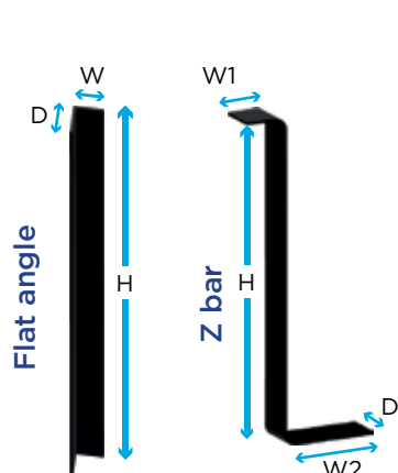
JBZ700 | TBK700
